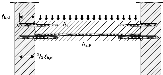
Figure 1: Overlap joint for rebar connections of slabs and beams
